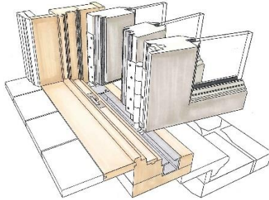
FOLDING DOOR
