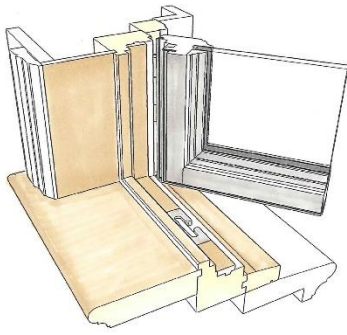
CASEMENT WINDOW
