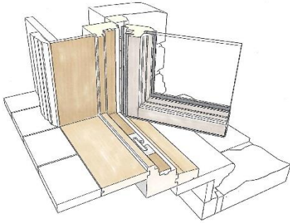
FRENCH DOOR
