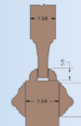
Recessed Molding W/ WB21 Bolection Classical Panel
