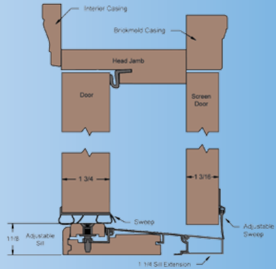
Non-Impact Prehang Details with Standard Jamb and Inswing Sill and Storm Door Attached
